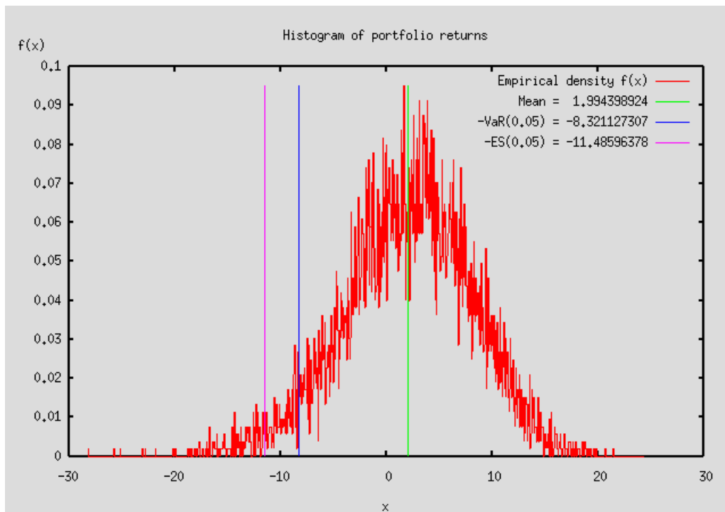
Figure 4: Histogram of returns; ES-optimized portfolio with 4 assets (local GS), 10^4 loops. Compared to the original portfolio in Figure 3, all values have significantly been improved (please note the different scales).
