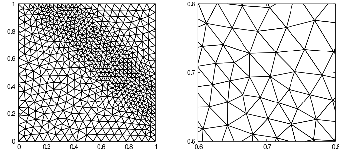
(c) Edge-based error estimator: 684 vertices and 1282 triangles, \|e\|_{L^2} = 1.4 \times 10^{-3} , maximum aspect ratio 3.8.
