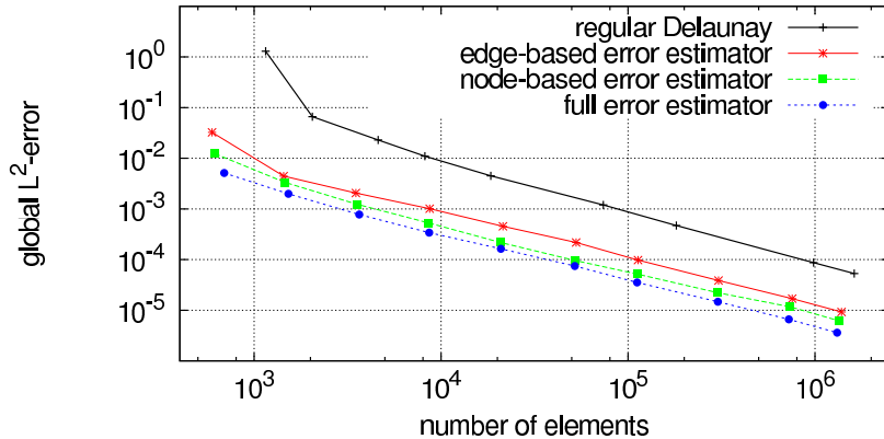
Figure 2: Example 5.1: a comparison of the error for adaptive finite element solutions obtained with mesh adaptation controlled by the reduced and full error estimators.
