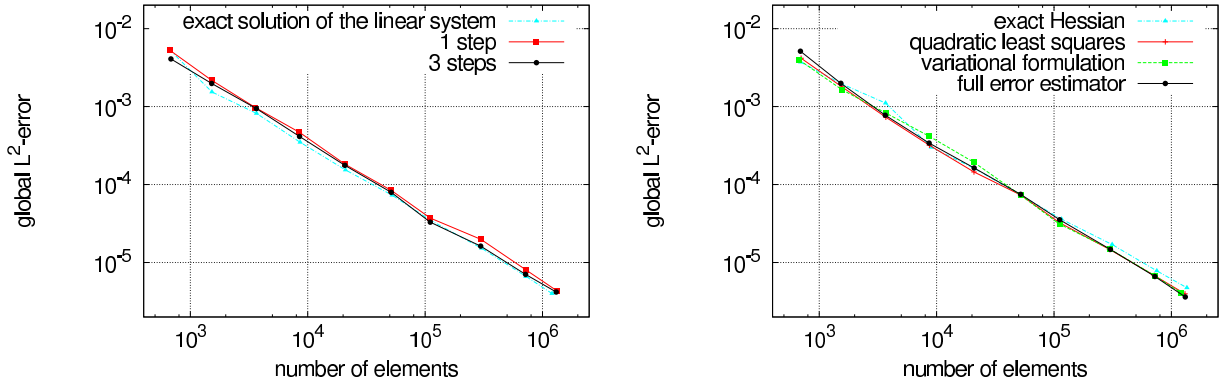
(a) Effects of the number of Gauß-Seidel iterations used in the solution of the linear system resulting from the error problem ( E_h ). (b) Error comparison for adaptive finite element solutions obtained with global error estimation and Hessian recovery.
