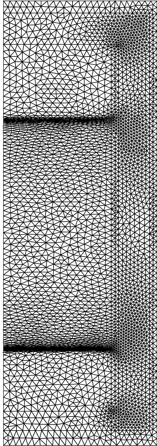
(b) Full error estimator: 3493 vertices and 6750 triangles, maximum aspect ratio 54.8, error estimate \|z_h\|_{L^2} = 4.2 \times 10^{-1} .
