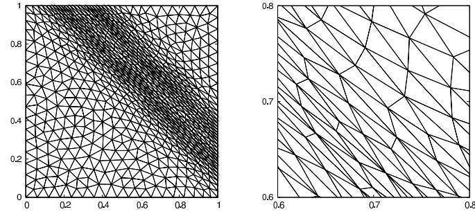
(d) Quadratic least squares Hessian recovery: 693 vertices and 1277 triangles, \|e\|_{L^2} = 3.5 \times 10^{-4} , maximum aspect ratio 13.5.
