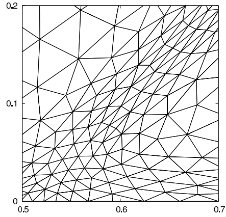
(a) Edge-based error estimator: 722 vertices and 1345 triangles, \|e\|_{L^2} = 5.0 \times 10^{-3} , maximum aspect ratio 12.8.
