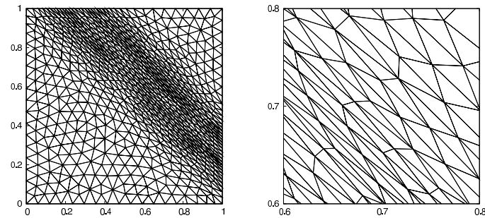
(e) Full error estimator: 714 vertices and 1318 triangles, \|e\|_{L^2} = 3.4 \times 10^{-4} , maximum aspect ratio 15.0.
