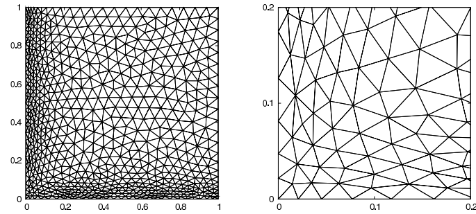
(c) Edge-based error estimator: 698 vertices and 1298 triangles, \|e\|_{L^2} = 3.0 \times 10^{-3} , maximum aspect ratio 7.0.
