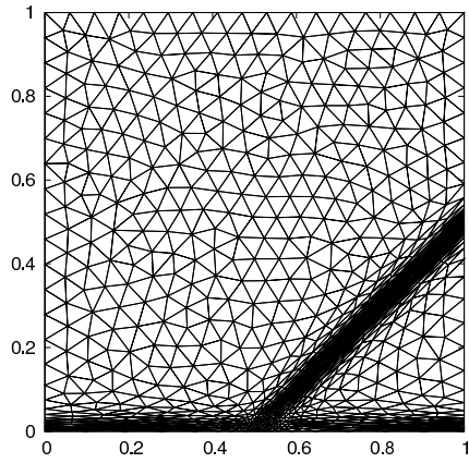
(c) Full error estimator: 763 vertices and 1413 triangles, \|e\|_{L^2} = 1.6 \times 10^{-3} , maximum aspect ratio 46.9.
