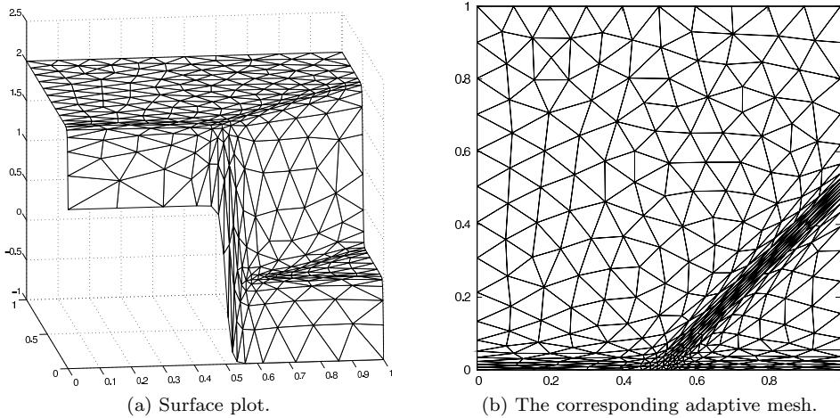
Figure 1: An example of anisotropic mesh adaptation for the test function u(x, y) = \tanh(60x) - \tanh(60(x - y) - 30) : Surface plot (a) of the function on an adaptive mesh (b) obtained with the use of the exact Hessian.
