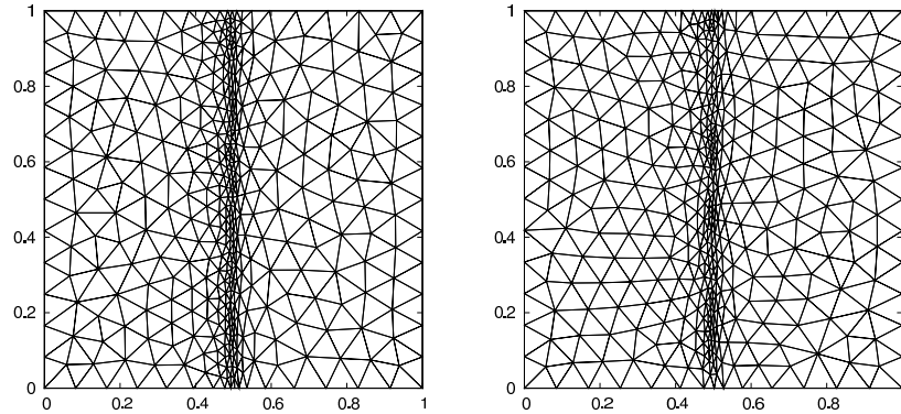
(b) Adaptation without predefined interface edges: quadratic least squares Hessian recovery, 385 vertices, \|e\|_{L^2} = 4.2 \times 10^{-3} , maximum aspect ratio 8.1 (left); full error estimator, 381 vertices, \|e\|_{L^2} = 4.1 \times 10^{-3} , maximum aspect ratio 7.1 (right).
