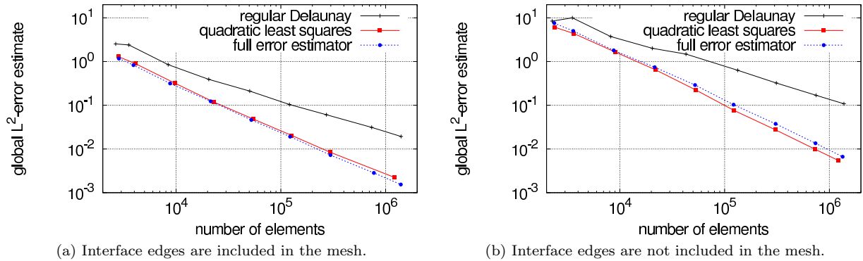
Figure 9: Heat conduction in a thermal battery: a comparison of the error for adaptive finite element solutions obtained on meshes (a) with and (b) without the interfaces being present in the mesh.
