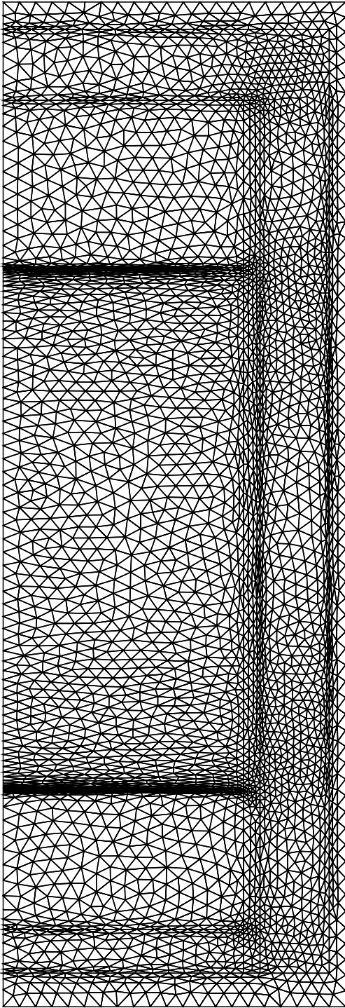
(a) Quadratic least squares Hessian recovery: 3499 vertices and 6781 triangles, maximum aspect ratio 39.2, error estimate \|z_h\|_{L^2} = 4.7 \times 10^{-1} .
