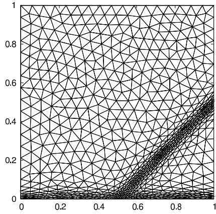
(b) Node-based error estimator: 720 vertices and 1339 triangles, \|e\|_{L^2} = 3.7 \times 10^{-3} , maximum aspect ratio 14.3.
