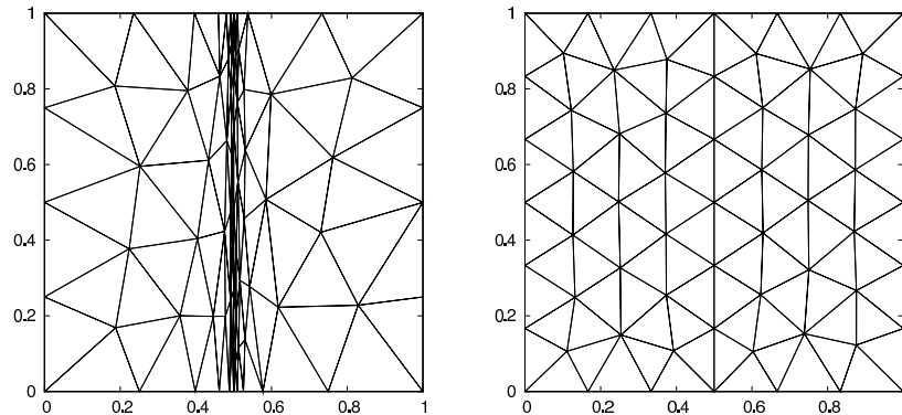
(c) Adaptation with predefined interface edges: quadratic least square Hessian recovery: 77 vertices, \|e\|_{L^2} = 3.1 \times 10^{-16} , maximum aspect ratio 60.7 (left); full error estimator, 63 vertices, \|e\|_{L^2} = 3.2 \times 10^{-16} , maximum aspect ratio 1.8 (right).
