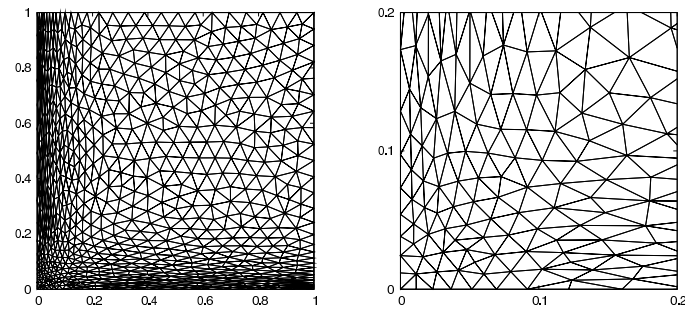
(e) Full error estimator: 712 vertices and 1332 triangles, \|e\|_{L^2} = 1.3 \times 10^{-3} , maximum aspect ratio 17.8.
