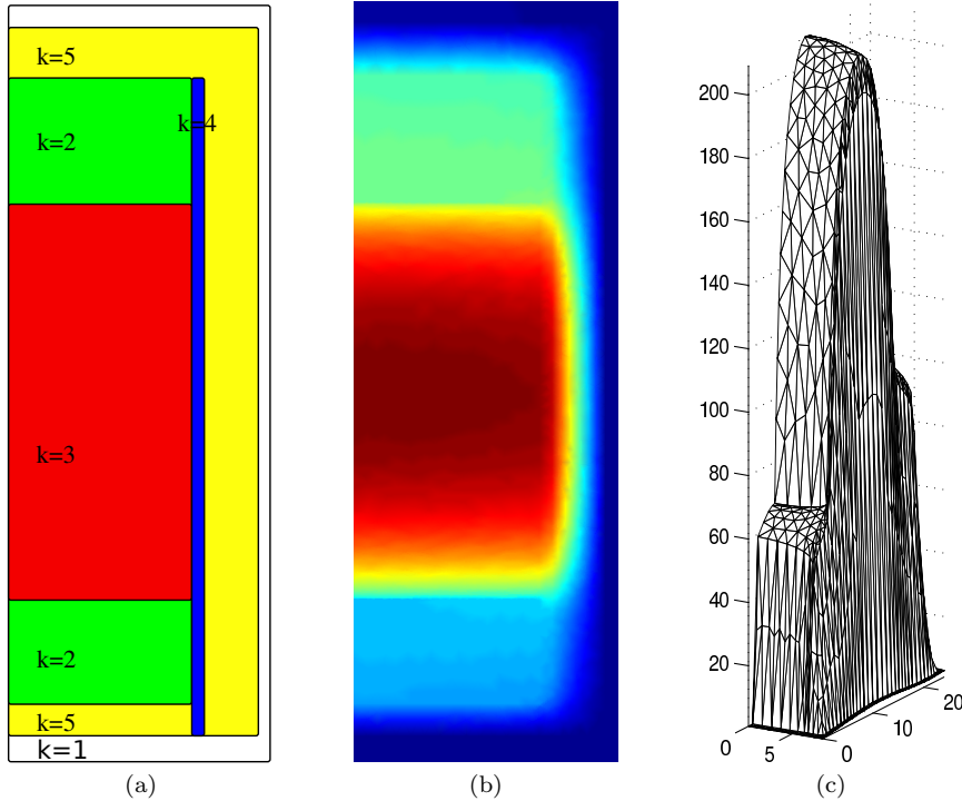
Figure 8: Heat conduction in a thermal battery: (a) device geometry, (b) contour plot, and (c) surface plot of a linear finite element solution.
