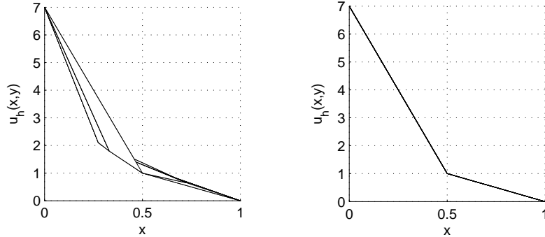
(a) Side views of finite element solutions: without the interface being present in the mesh, the solution is non-planar and not exact (left, different lines represent the solution for different values of y ); with the interface being present in the mesh, the solution is exact (right).
