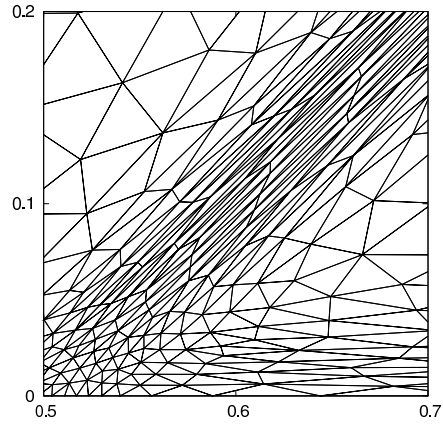
(c) Full error estimator: 763 vertices and 1413 triangles, \|e\|_{L^2} = 1.6 \times 10^{-3} , maximum aspect ratio 46.9.
