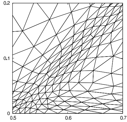
(b) Node-based error estimator: 720 vertices and 1339 triangles, \|e\|_{L^2} = 3.7 \times 10^{-3} , maximum aspect ratio 14.3.
