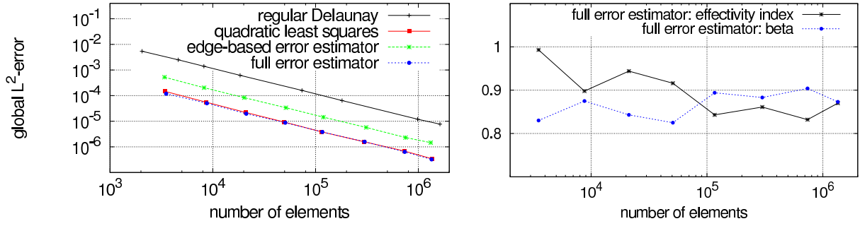
(a) Error comparison for adaptive solutions.
