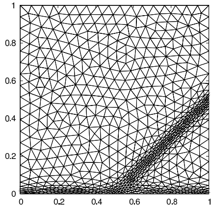
(a) Edge-based error estimator: 722 vertices and 1345 triangles, \|e\|_{L^2} = 5.0 \times 10^{-3} , maximum aspect ratio 12.8.
