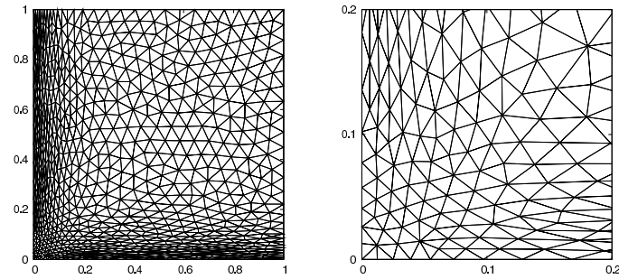
(d) Quadratic least squares Hessian recovery: 710 vertices and 1327 triangles, \|e\|_{L^2} = 1.3 \times 10^{-3} , maximum aspect ratio 20.0.
