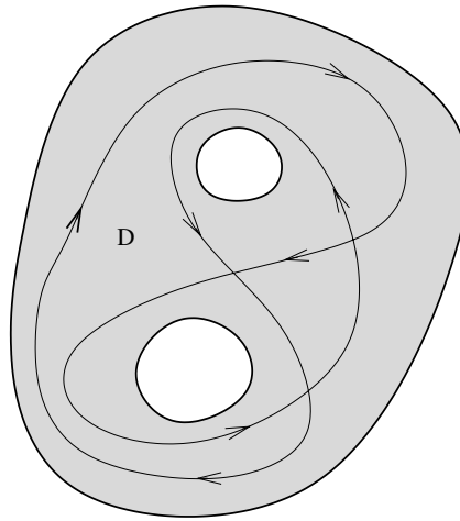
Figure 8.3: A closed path that is D -homologous to zero
