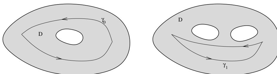
Figure 8.4: A path that is not null-homotopic in D on the left and a path that is null-homotopic in D on the right.
